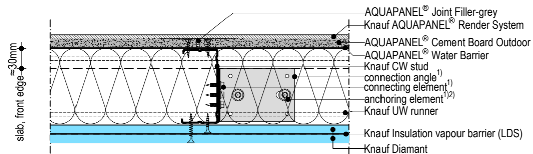
H1 Horizontal section - board joint
