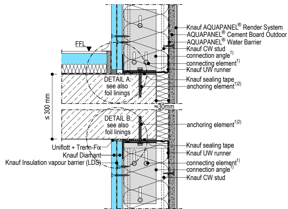
V1 Vertical section - connection to end plate
