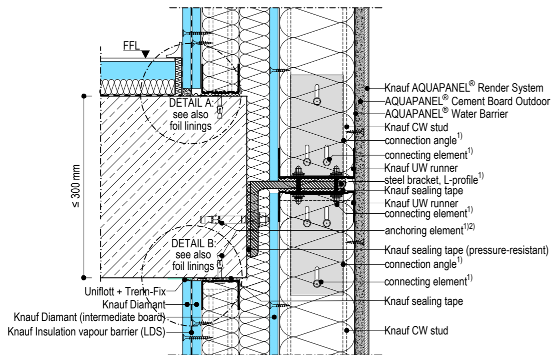
V1 Vertical section - connection to end plate
