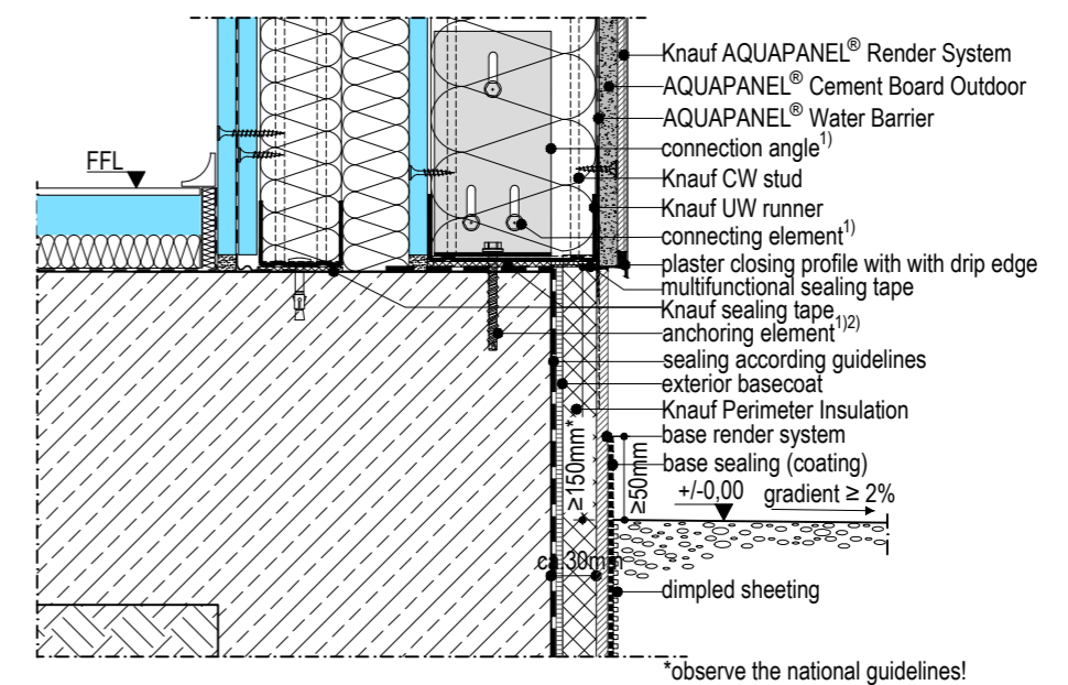
V2 Vertical section - connection to base
