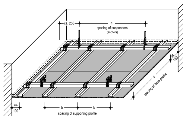
Base Profile and Supporting Profile / suspended
