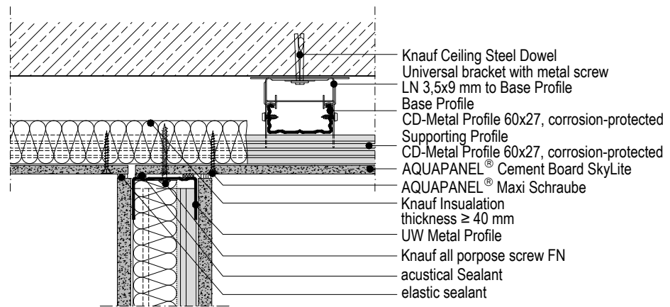
KNAUF Connection wall to suspended ceiling
