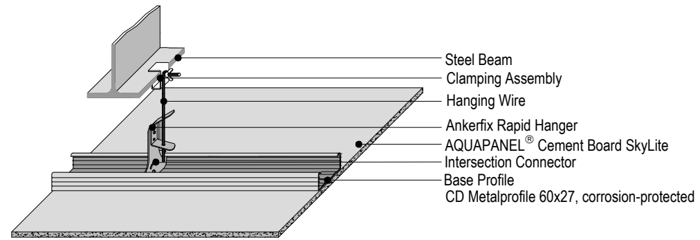
knapp Isometry ceiling, connection steel beam
