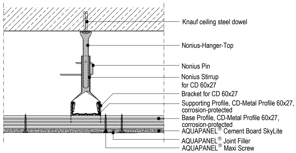
Vertical section with longitudinal joint
