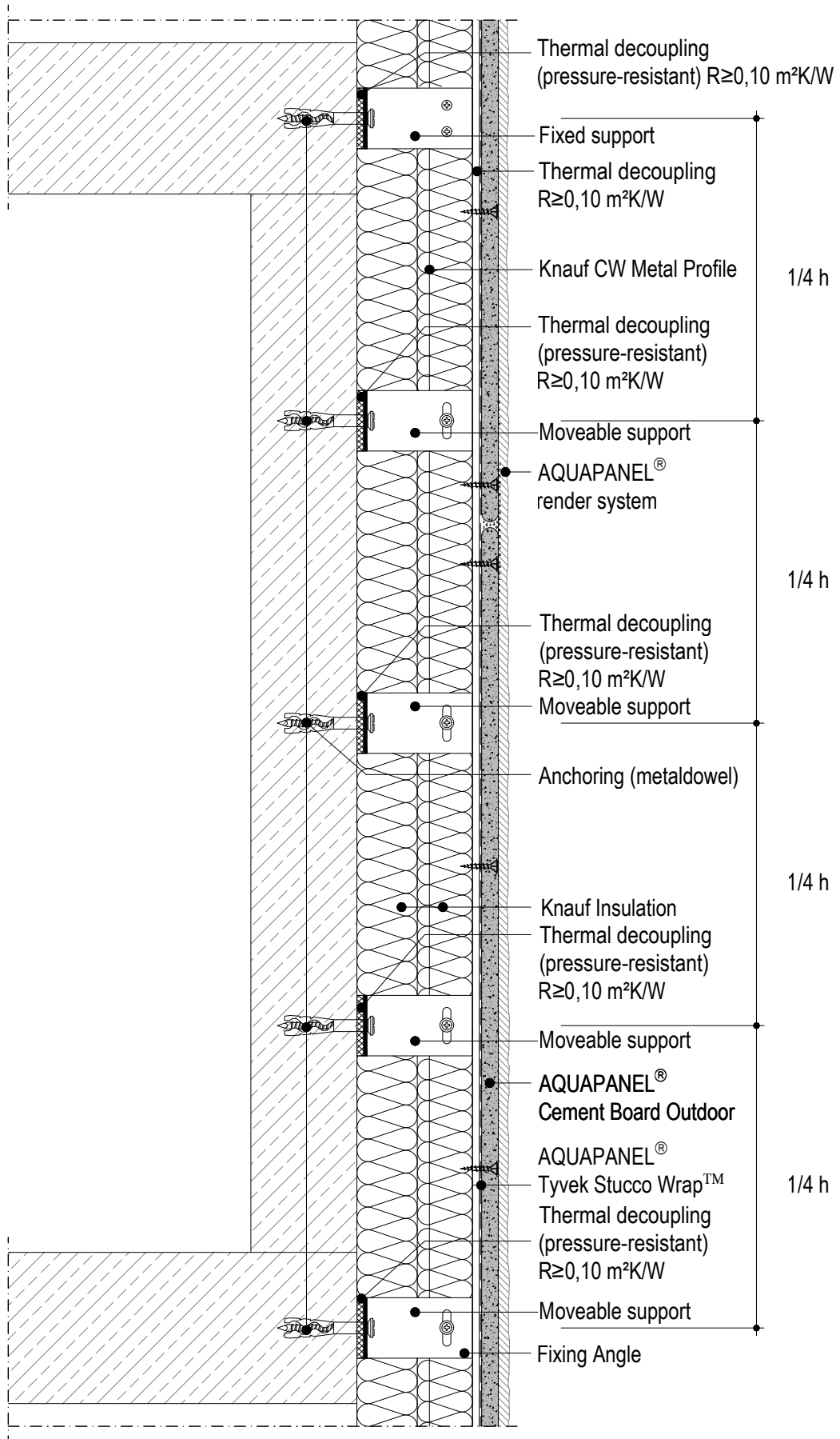
W638E-V1.en Vertical section
