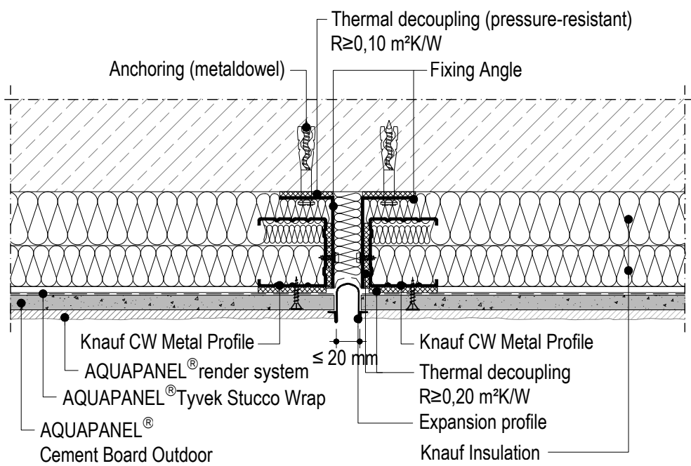
KNAUF W682-BFU1.en Expansion joint
