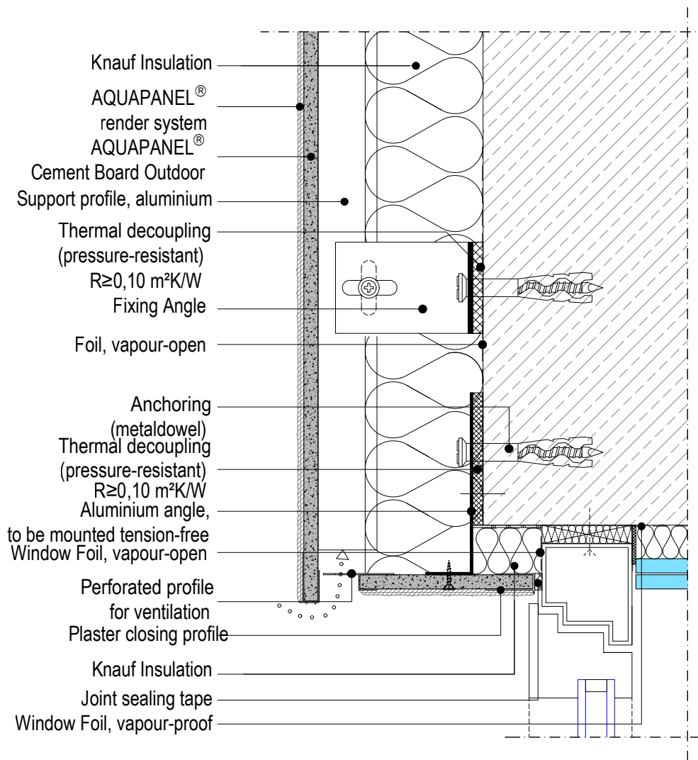
KNAUF W684T-FE-VO1.en Upper window connection
