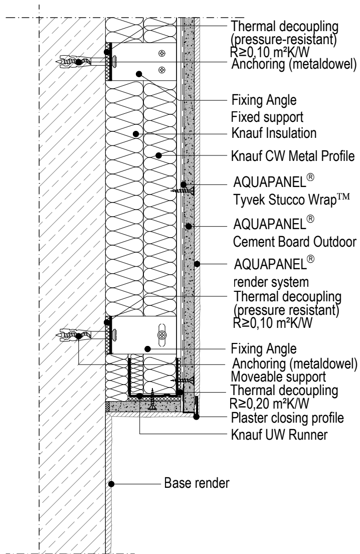
KNAUF W684T-SO-V2.en Foot point, option 2
