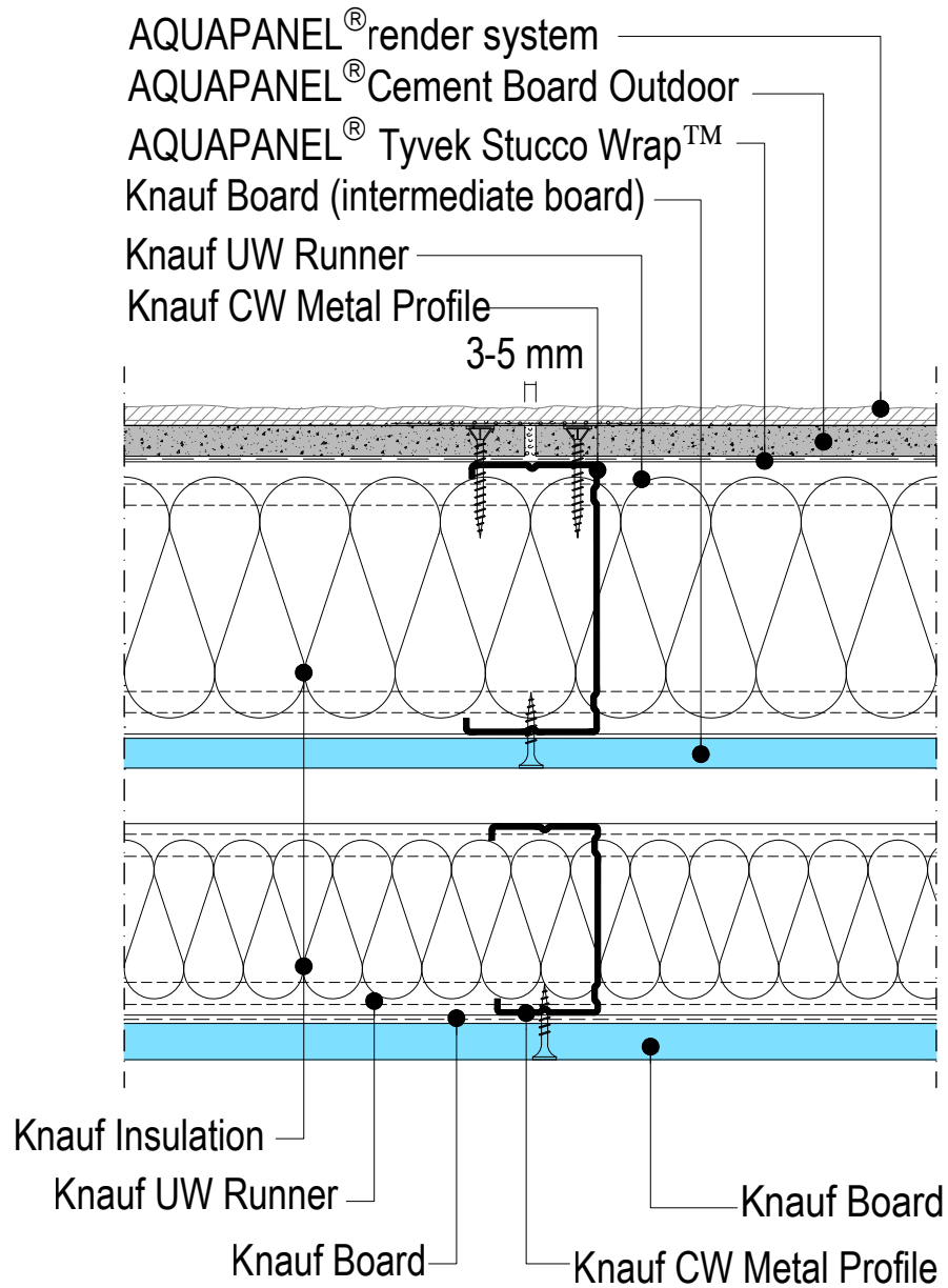
W 387E-B1.en Cross section with joint
