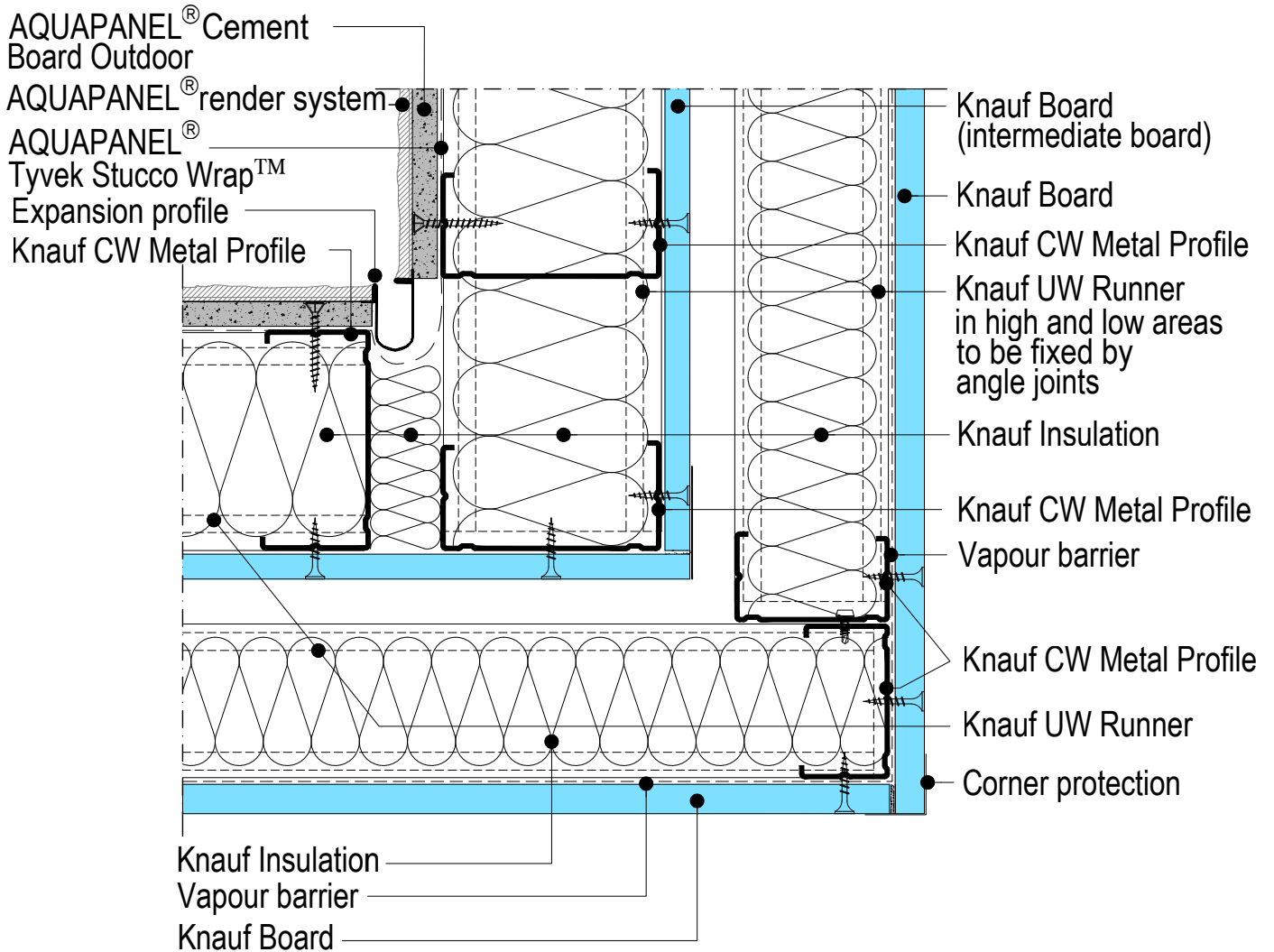
W387E-DBFU1.en Inside corner with dilatation joint
