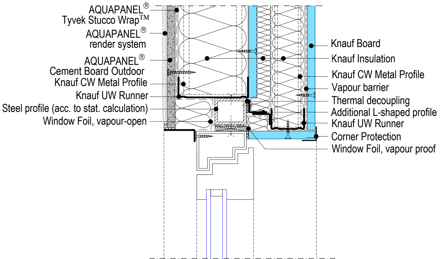
W387E-FE-VO2.en Upper connection to window, option 2
