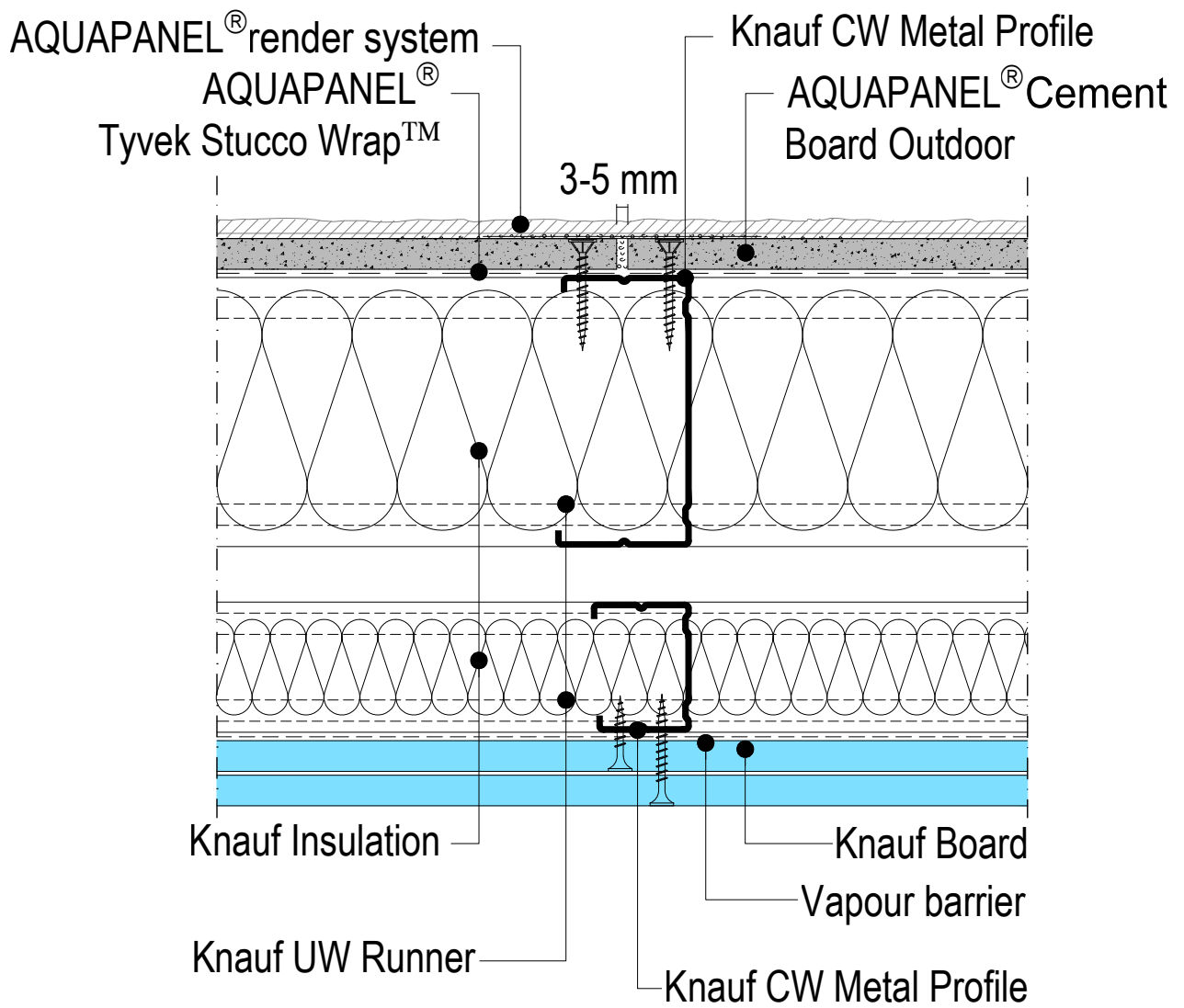
W388E-B1.en Cross section with joint
