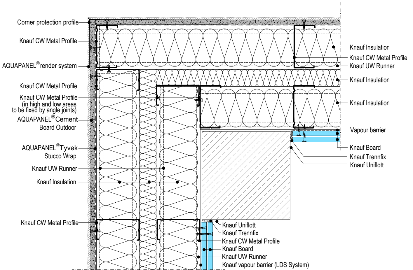
W388E-ES1.en Outside corner, horizontal section
