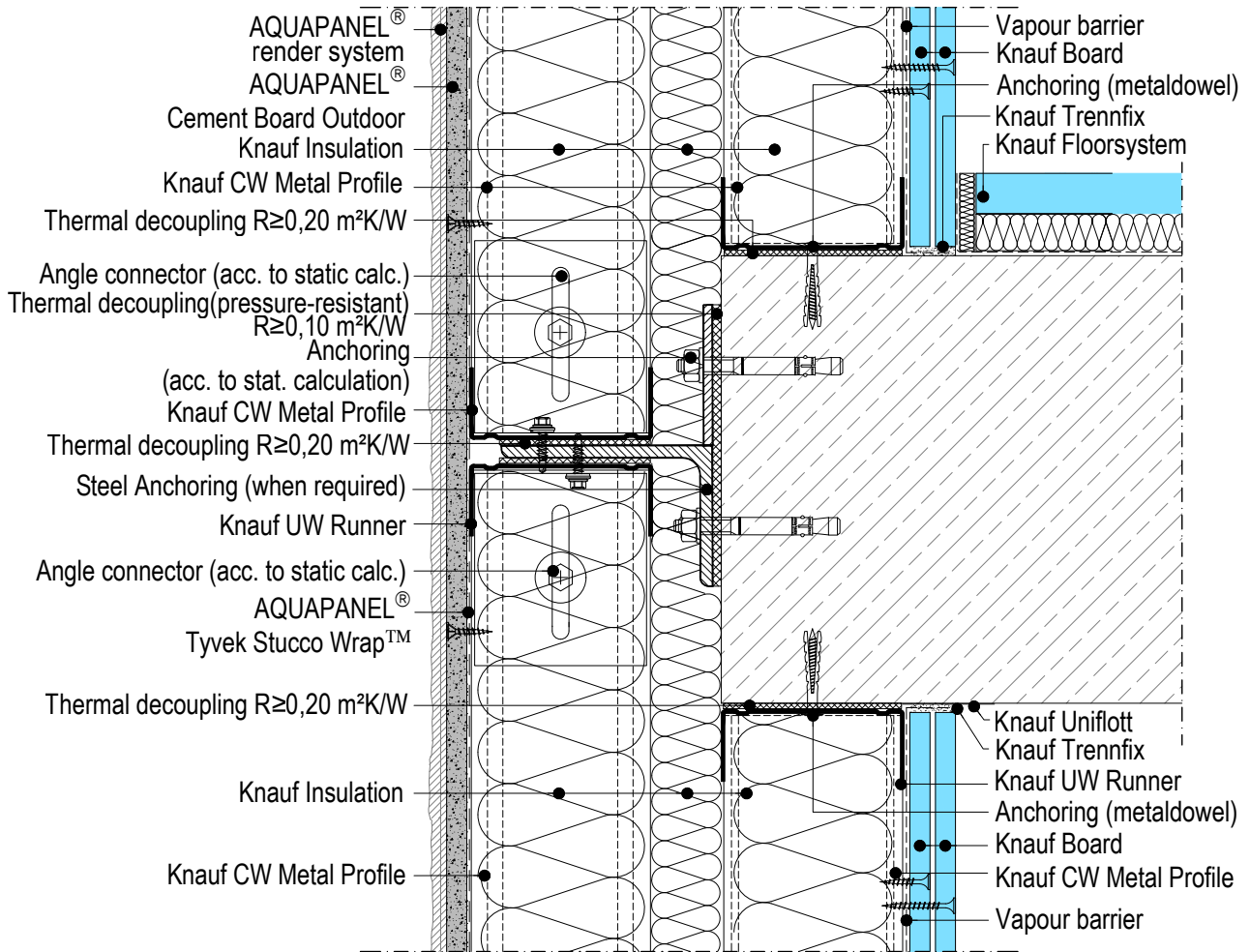
W388E-VM2.en Connection to ceiling: Steel angle and anchoring, option 2
