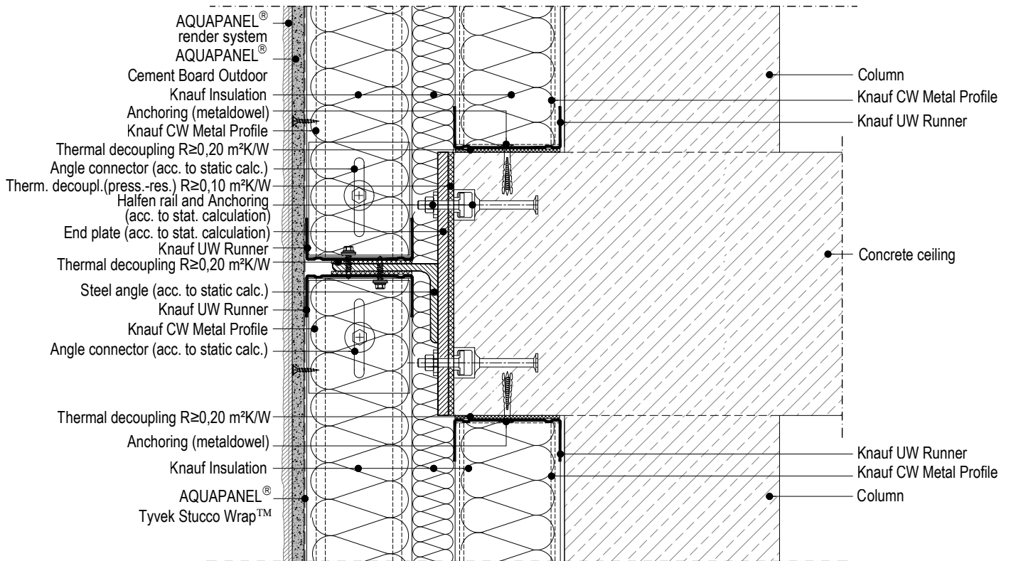
W388E-VMS1.en Connection to ceiling: Steel angle and end plate with connection to column, option 3
