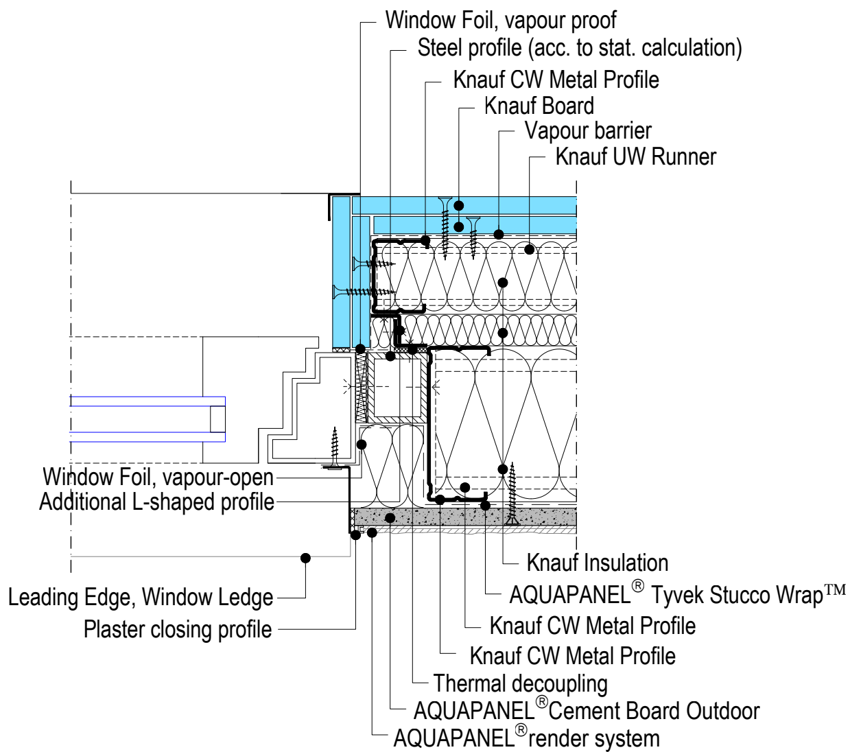
W388E-FE-VM2.en Side connection to window, option 1
