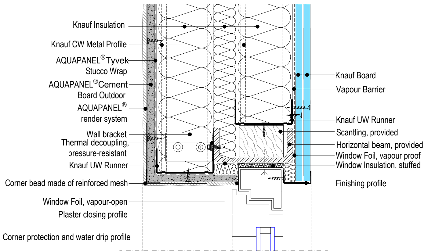
KNAUF W388E-FE-VO1_b.en Connection to window lintel
