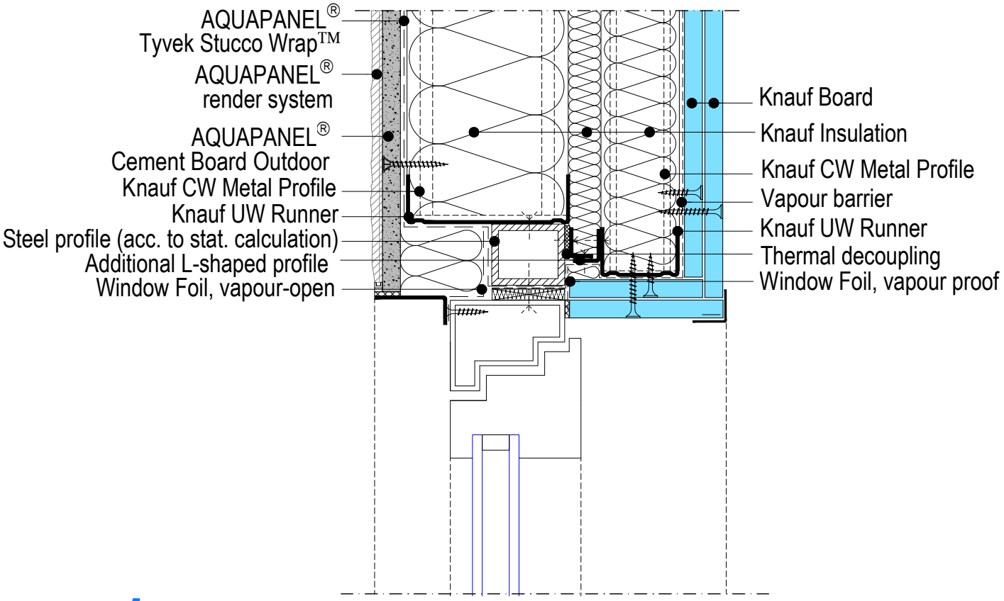
W388E-FE-VO2.en Upper connection to window, option 2
