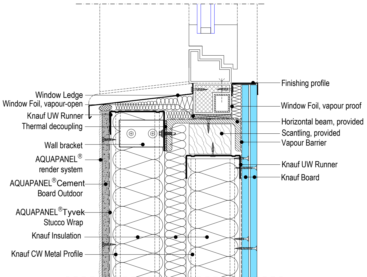
KNAUF W388E-FE-VU1_b.en Connection to window ledge
