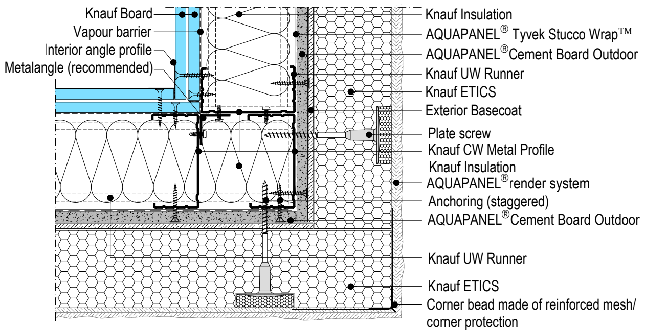
W384E-E-ETICS1.en Outside corner with Knauf ETICS
