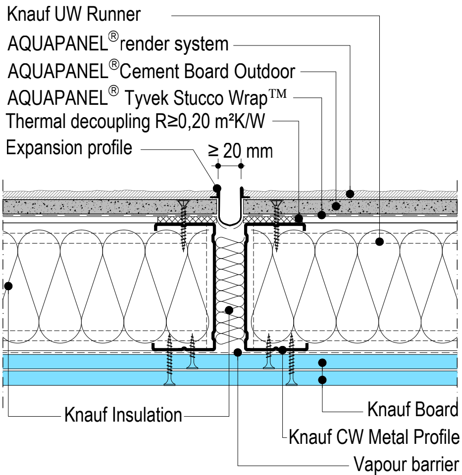
KNAUF W 384E-BFU1.en Essential dilatation joint (vertical) in outside areas (located every 15 m)
