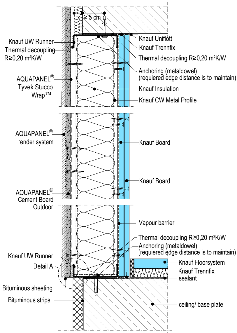
knauf W 384E-V1.en Vertical cross section, option 1
