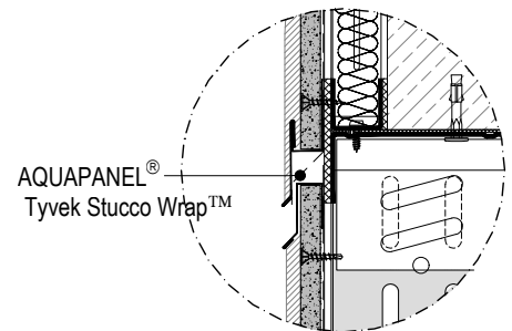
Detail A: water barrier in joint area
