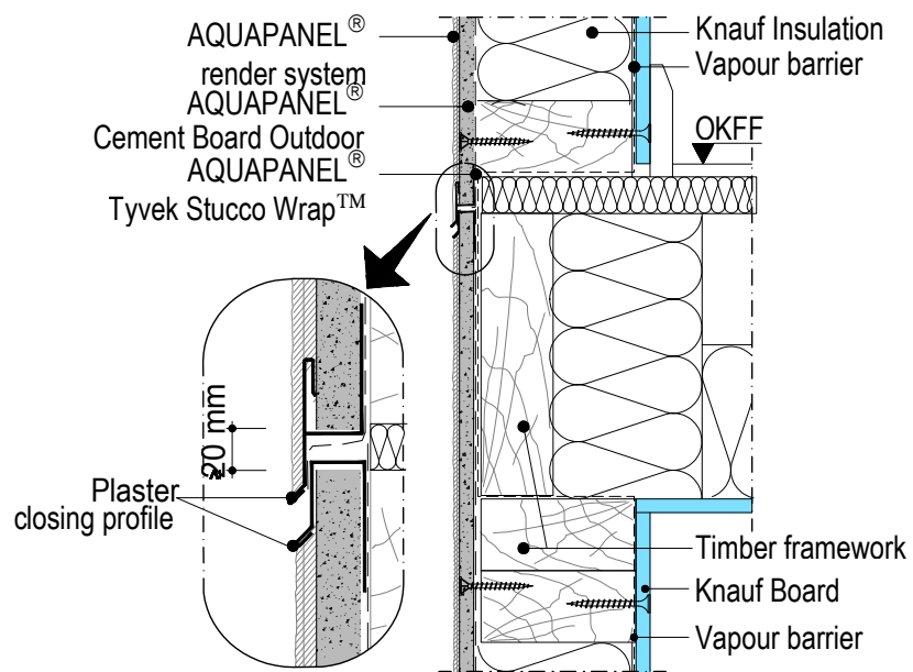
KNAUF W573-VM1.en Horizontal dilation joint (floor slabs)
