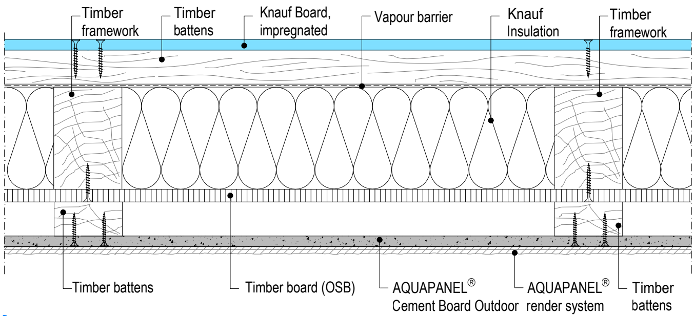
W681-H1.en Horizontal Section
