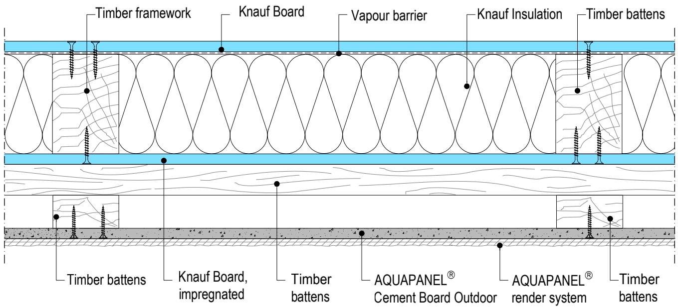
W681-H2.en Horizontal Section
