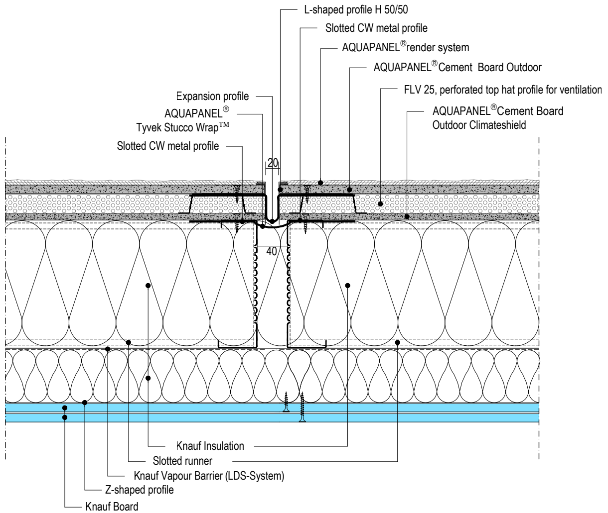
W684W-BFU1.en Horizontal cross section with expansion joint
