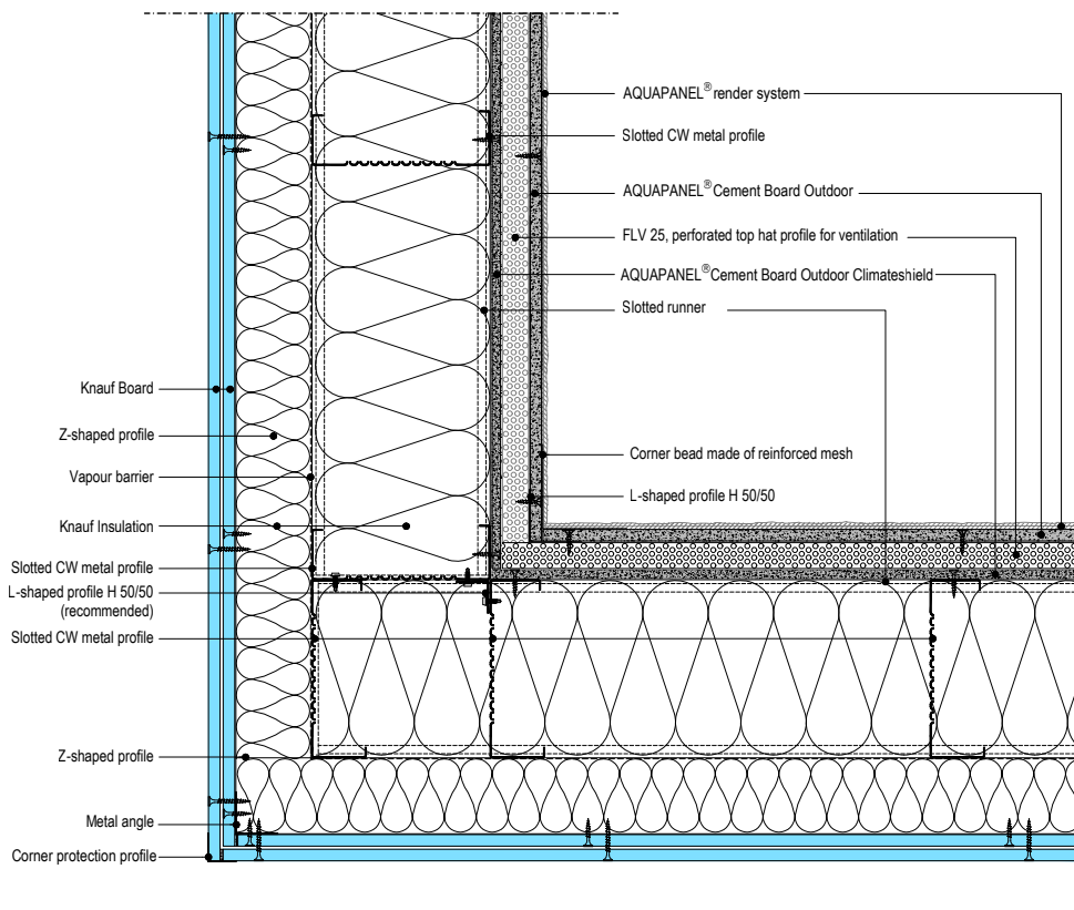
KNAUF W684W-D1.en Back-ventilated facade with inside corner, without expansion joint
