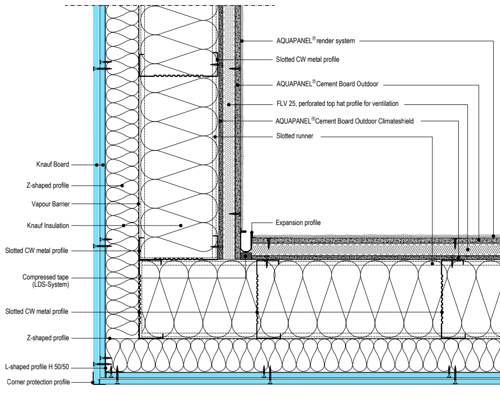
knauf W684W-DBFU1.en Inside corner with expansion profile
