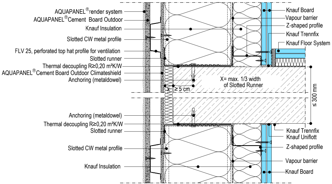
W684W-VM1.en Vertical cross section
